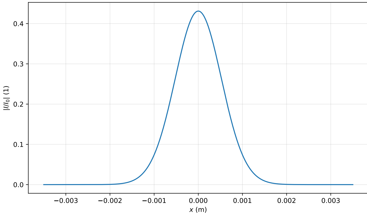
Intensity profile I(x, y = 0, z = 2.468m)/I_0 , P_{in}=0.1P_{cr} , artificial time
